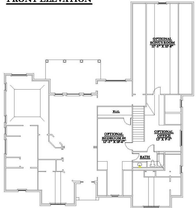
OPTIONAL SECOND FLOOR PLAN
