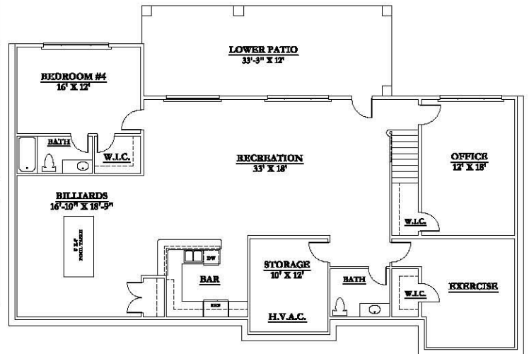
OPTIONAL BASEMENT PLAN BASEMENT HEATED: 2173 SQ. FT.
